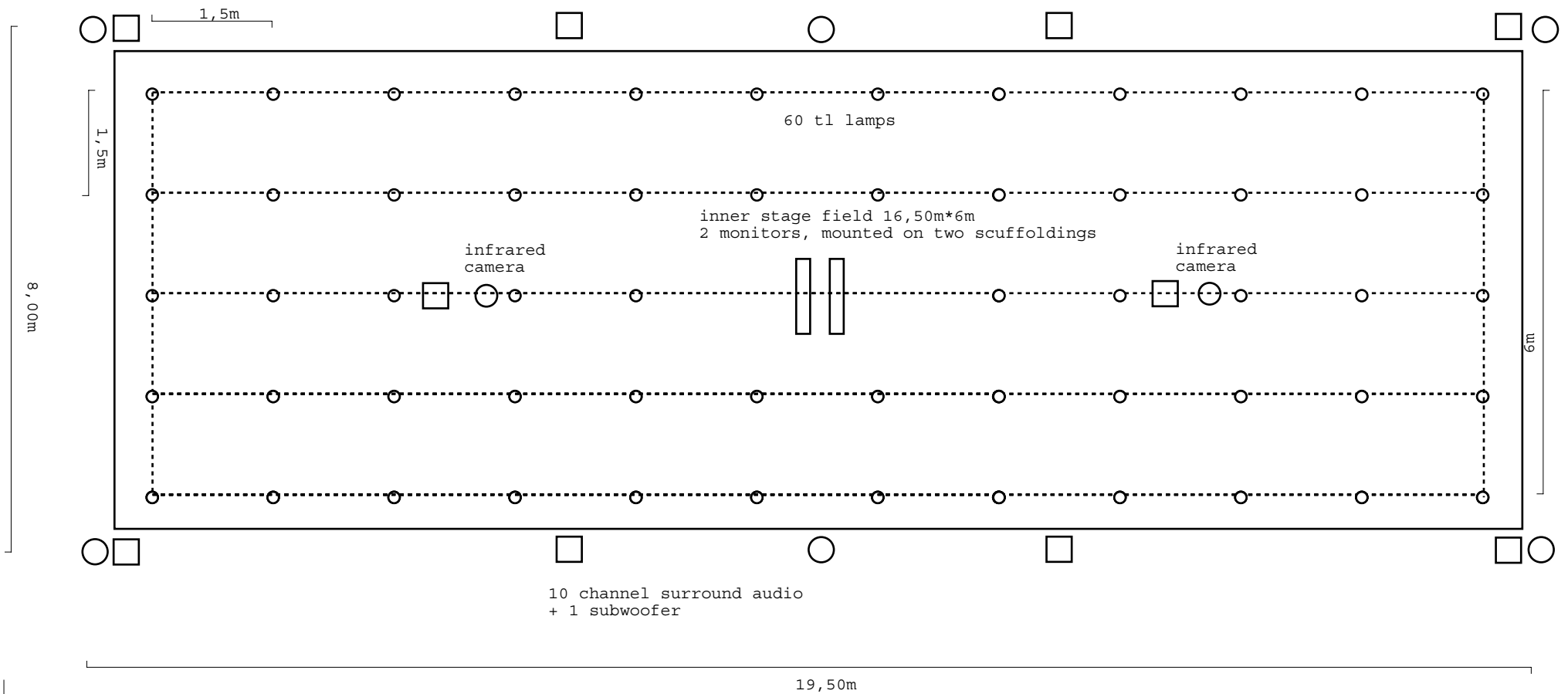
forest 2 - floorplan
